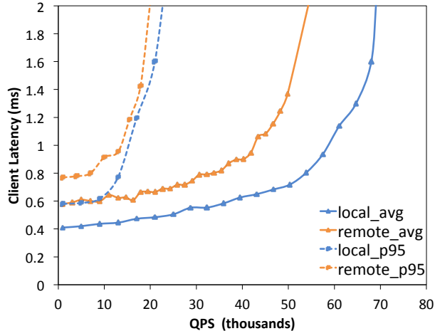
(b) For a single SSD server, remote vs. local Flash decreases client QPS by 20% on average. The percentage overhead is 10% for requests at the tail.
